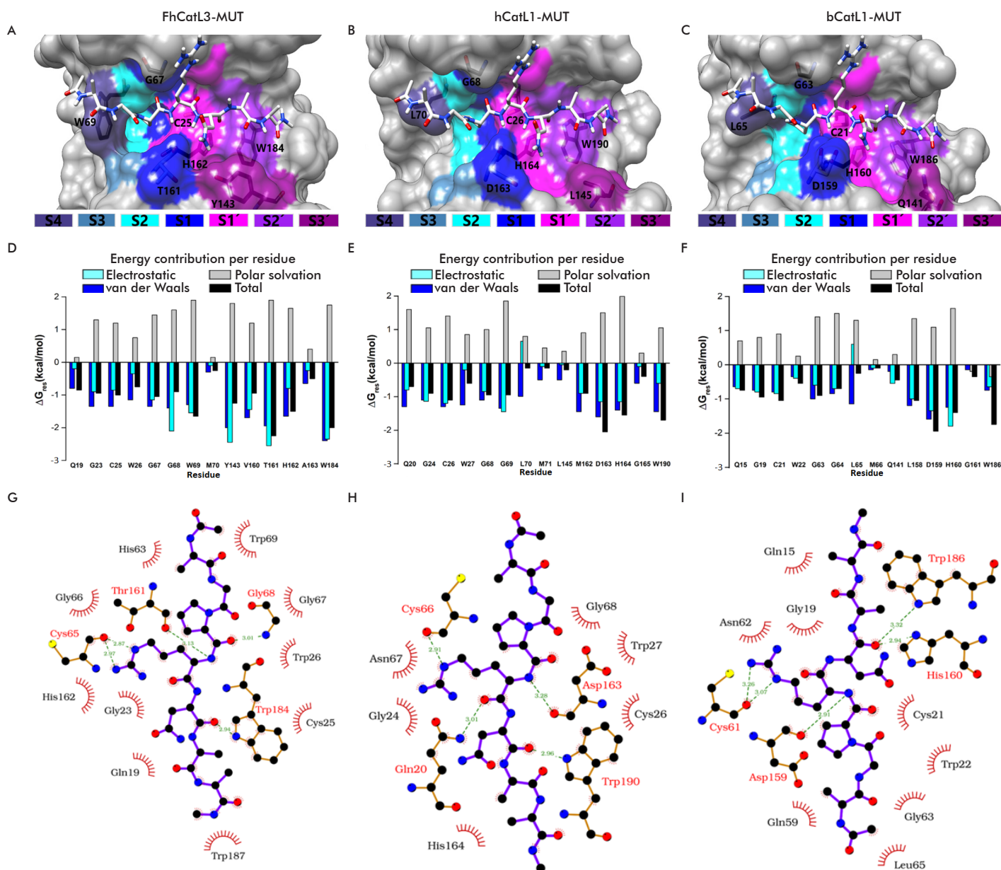
Figure 2. Representation of the interaction interface of compound HTS12701 with Fasciola hepatica cathepsin L3 (FhCatL3; A, D, G), human cathepsin L1 (hCatL1; B, E, H) and bovine cathepsin L1 (bCatL1; C, F, I). A-C) The subsites were colored according to the legend. D-F) The energy decomposition per residue was calculated considering the van der Waals, electrostatic, polar solvation and total contributions. G-I) The respective protein-ligand interaction diagrams obtained in LigPlot show apolar contacts as red jagged arcs and polar (H-bonds) as green dashed lines.
