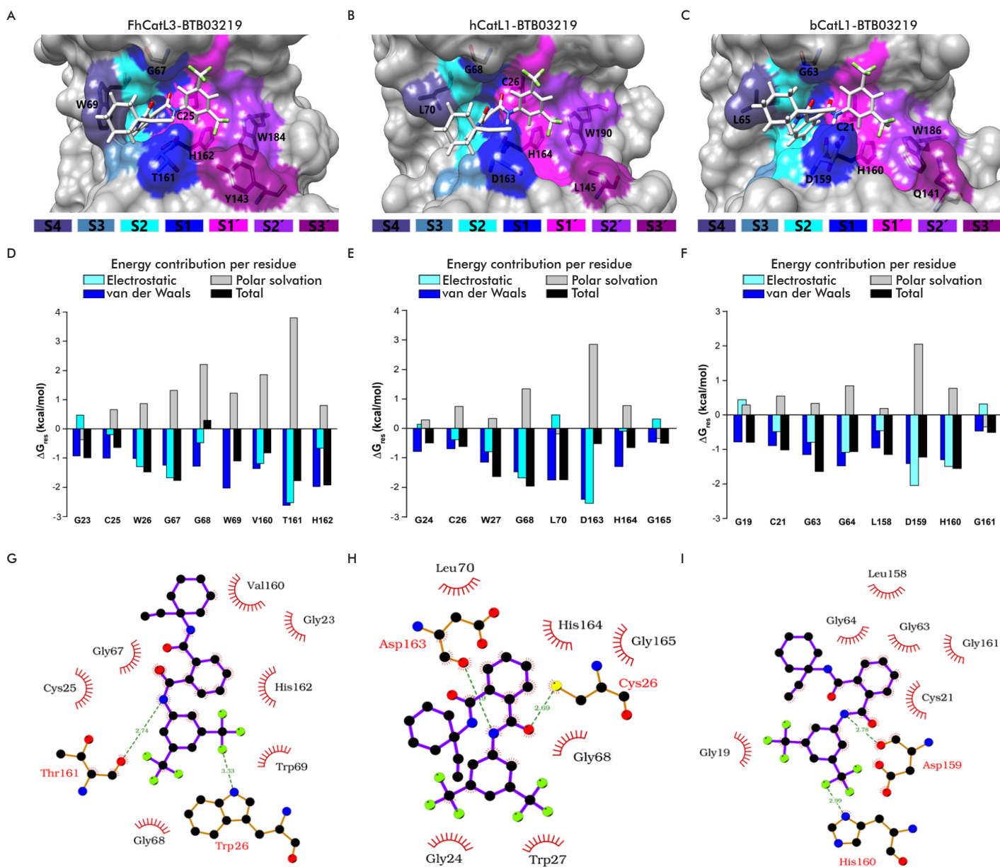
Figure 5. Representation of the interaction interface of compound BTB03219 with Fasciola hepatica cathepsin L3 (FhCatL3; A, D, G), human cathepsin L1 (hCatL1; B, E, H) and bovine cathepsin L1 (bCatL1; C, F, I). A, B and C) The subsites were colored according to the legend. D, E and F) The energy decomposition per residue was calculated considering the van der Waals, electrostatic, polar solvation and total contributions. G, H and I) The respective protein-ligand interaction diagrams obtained in LigPlot show apolar contacts as red jagged arcs and polar (H-bonds) as green dashed lines.
