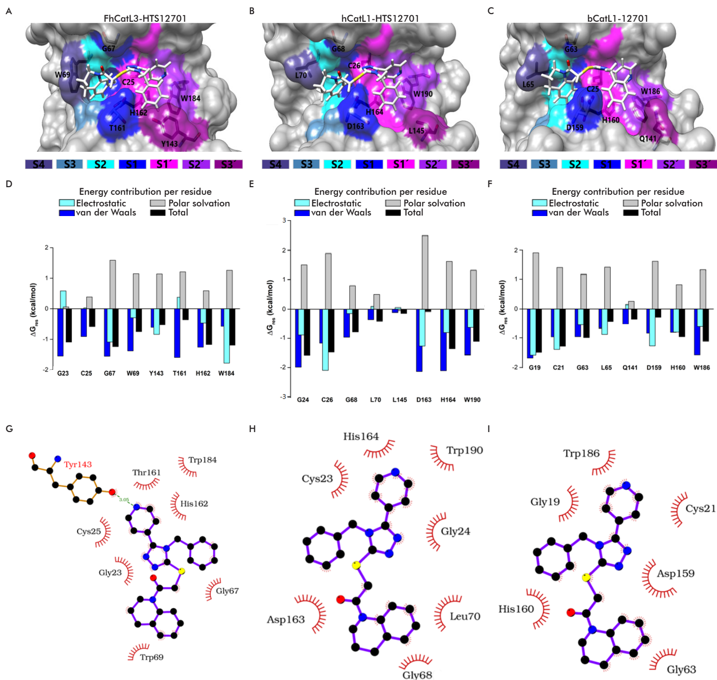
Figure 4. Representation of the interaction interface of compound HTS12701 with Fasciola hepatica cathepsin L3 (FhCatL3; A, D, G), human cathepsin L1 (hCatL1; B, E, H) and bovine cathepsin L1 (bCatL1; C, F, I). A, B and C) The subsites were colored according to the legend. D, E and F) The energy decomposition per residue was calculated considering the van der Waals, electrostatic, polar solvation and total contributions. G, H and I) The respective protein-ligand interaction diagrams obtained in LigPlot show apolar contacts as red jagged arcs and polar (H-bonds) as green dashed lines.
