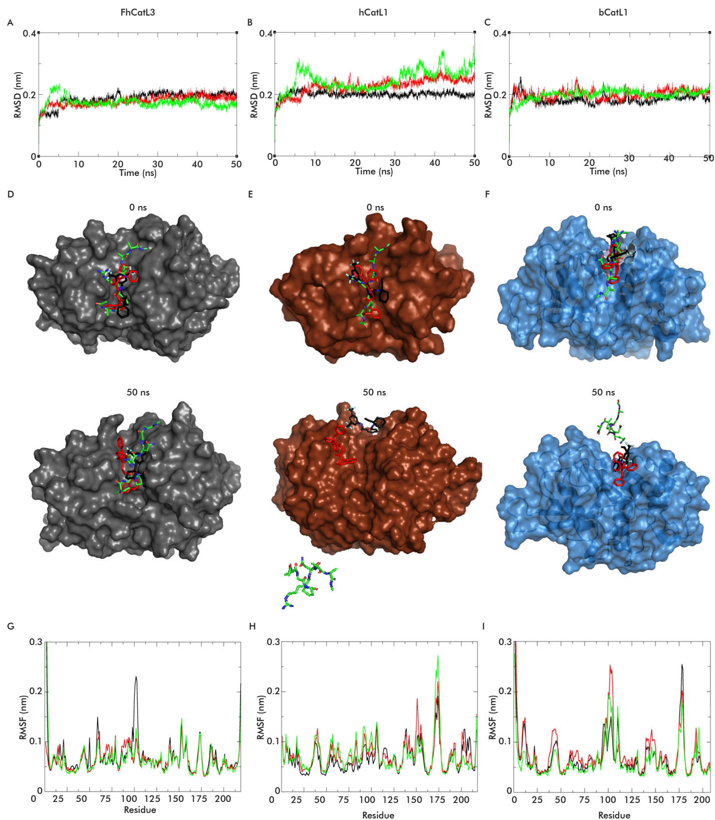
Figure 3. Variations of the root-mean-square deviation in distance (RMSD) of the atoms of the protein-ligand complexes and the root root-mean-square fluctuation (RMSF) per residue for the nine systems. A-C) RMSD analysis from 0 to 50 ns. D-F) Molecular dynamics of the protein-ligand complex and the inhibitor at 0 and 50 ns. G-I) RMSF analysis. Ligands are color-coded (A-C, G-I): BTB03219 (black), HTS12701 (red), and MUT peptide (green).
