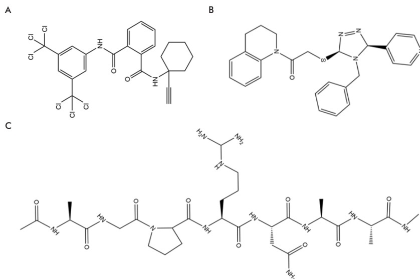
Figure 1. 2D structure of the three ligands used to analyze the Fasciola hepatica cathepsin L3 off-targets interactions with two potential inhibitors. A) The BTB03219 non-peptide inhibitor. B) The HTS12701 non-peptide inhibitor. C) The peptide mimetic (MUT) of amino acidic sequence ACE-AGPR↓NAA-NME
